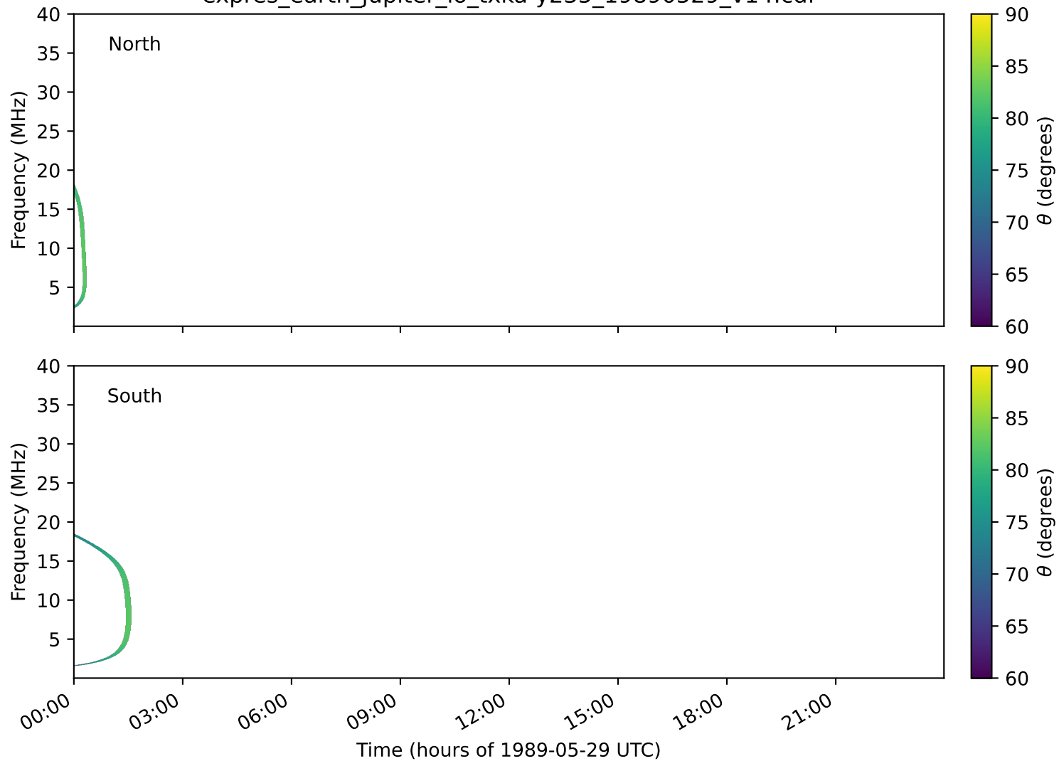
expres_earth_jupiter_io_txka-y235_19890529_v14.cdf
