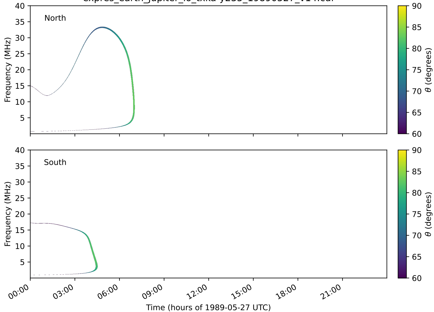
expres_earth_jupiter_io_txka-y235_19890527_v14.cdf
