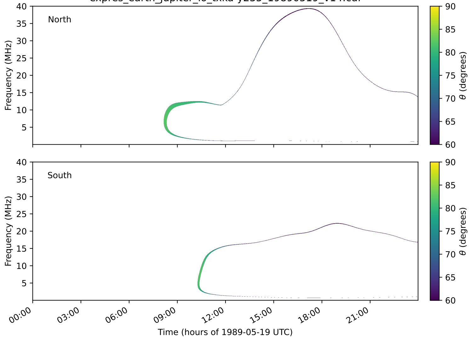
expres_earth_jupiter_io_txka-y235_19890519_v14.cdf
