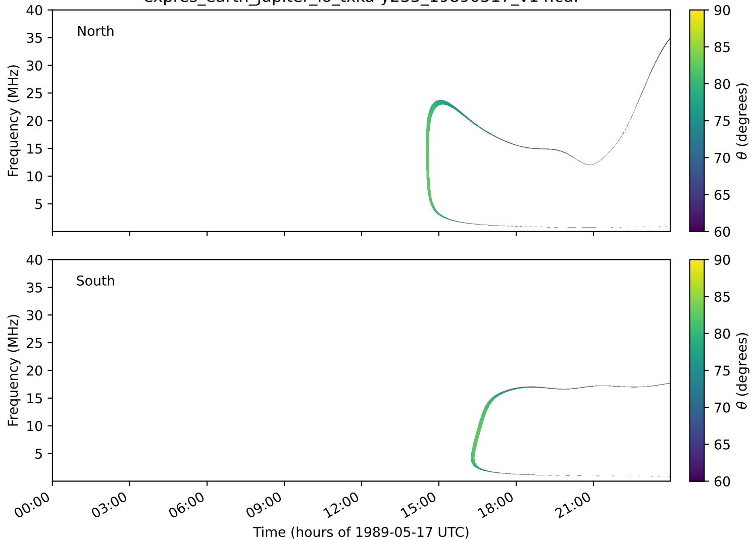
expres_earth_jupiter_io_txka-y235_19890517_v14.cdf
