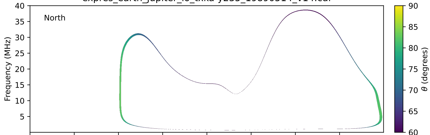
expres_earth_jupiter_io_txka-y235_19890514_v14.cdf
