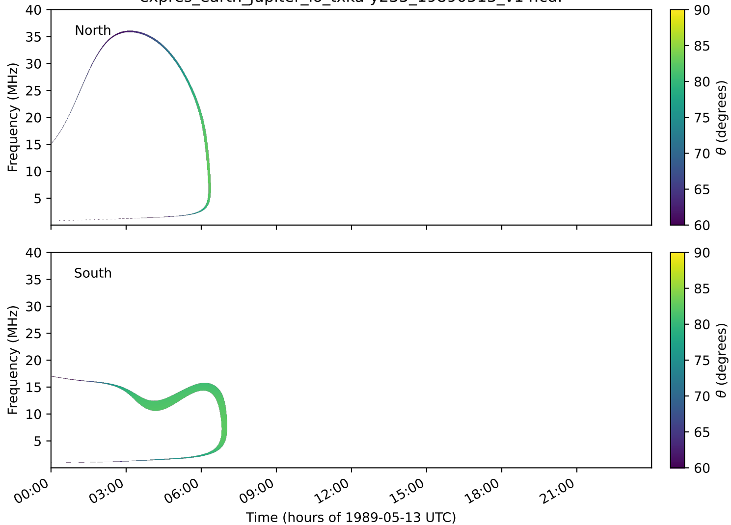
expres_earth_jupiter_io_txka-y235_19890513_v14.cdf
