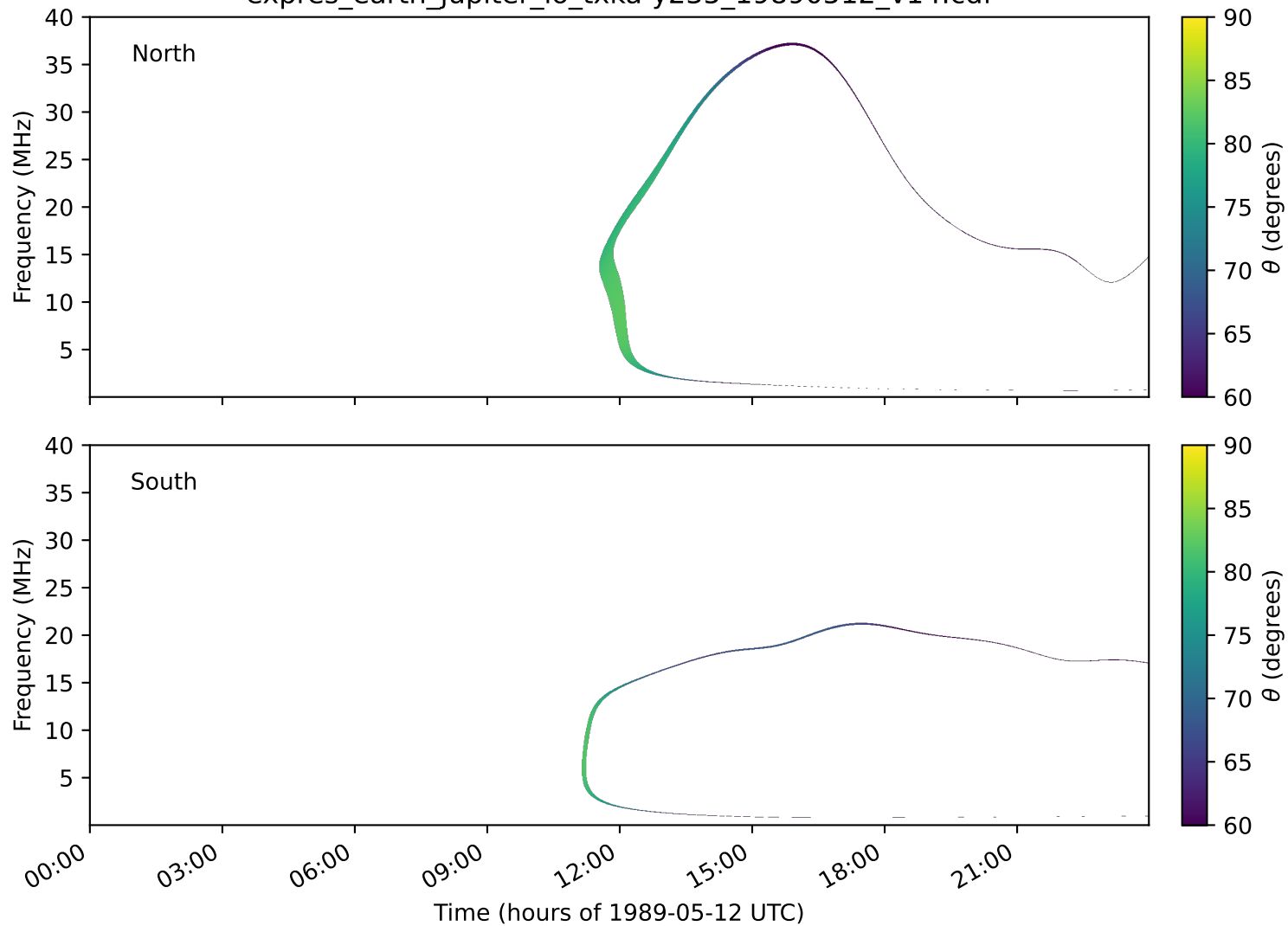
expres_earth_jupiter_io_txka-y235_19890512_v14.cdf
