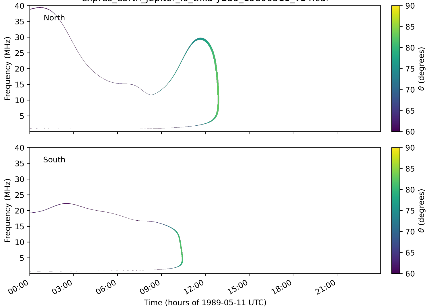
expres_earth_jupiter_io_txka-y235_19890511_v14.cdf
