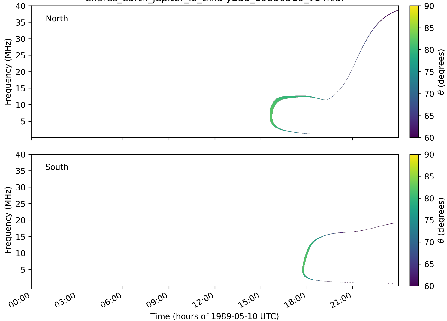
expres_earth_jupiter_io_txka-y235_19890510_v14.cdf
