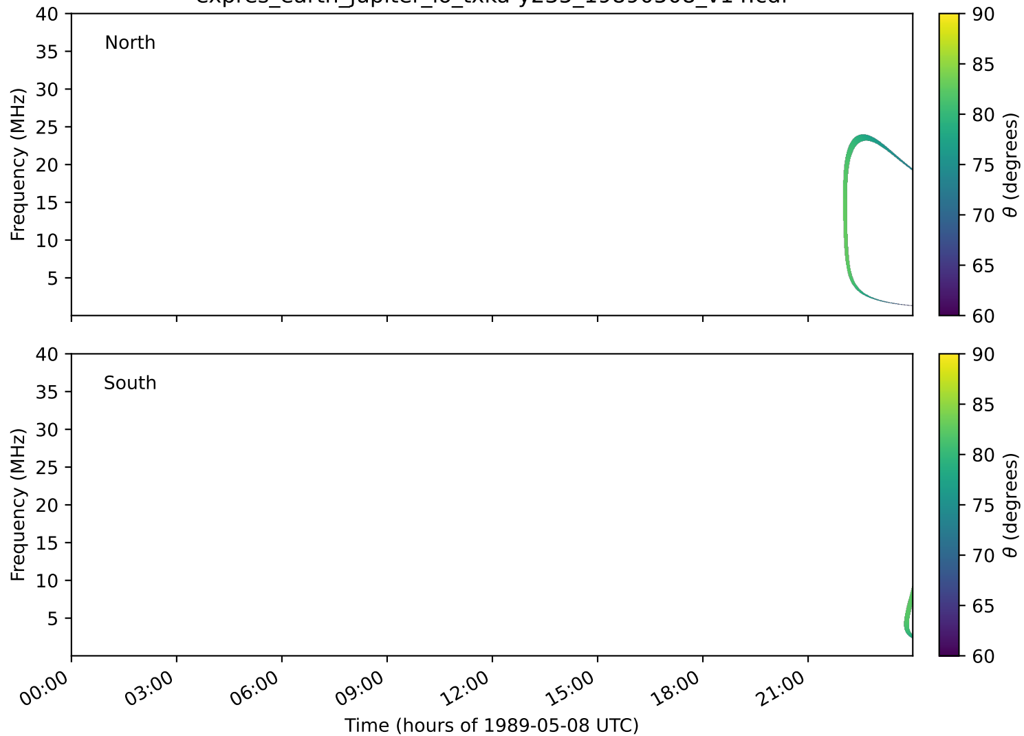
expres_earth_jupiter_io_txka-y235_19890508_v14.cdf
