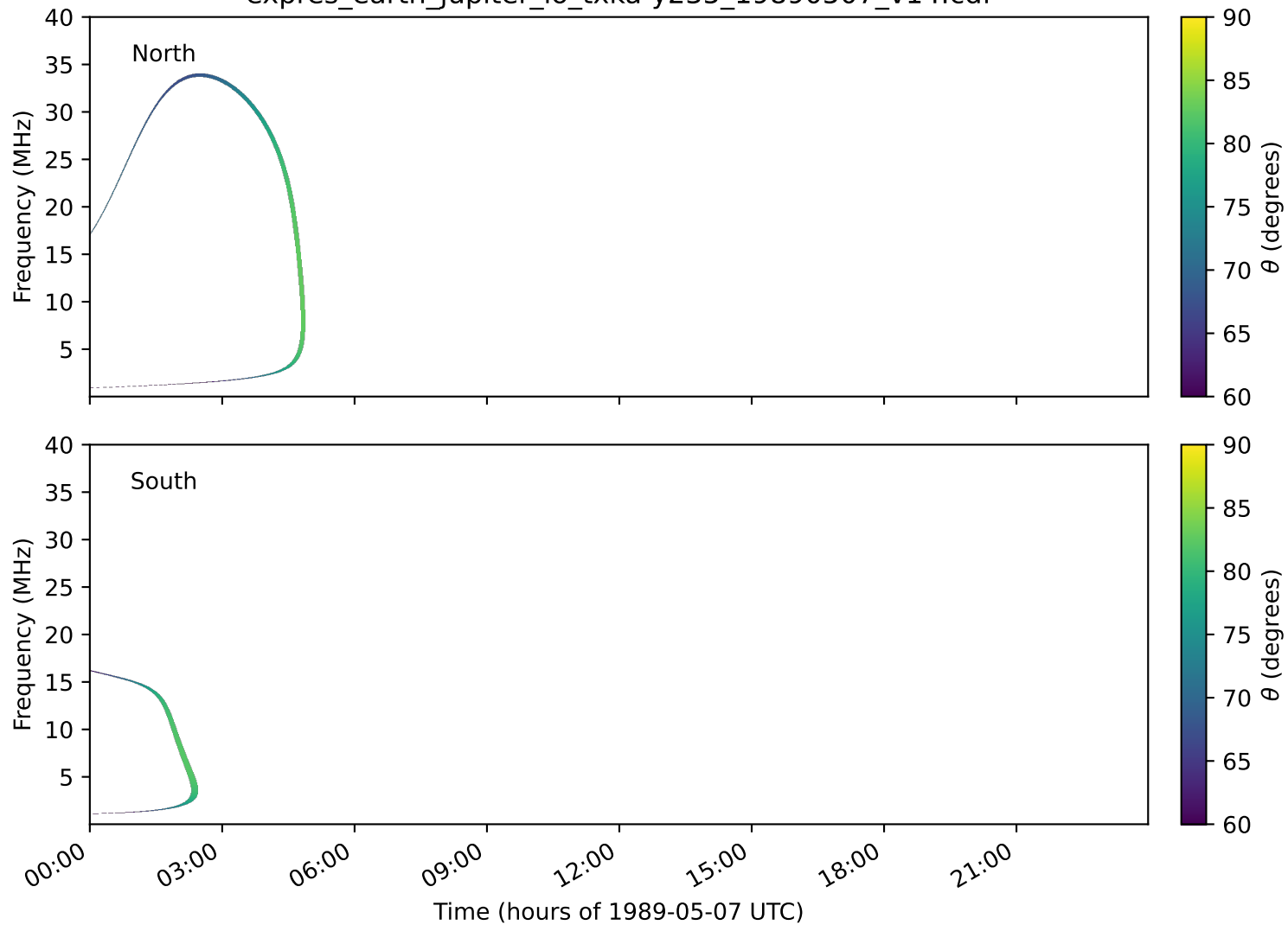
expres_earth_jupiter_io_txka-y235_19890507_v14.cdf
