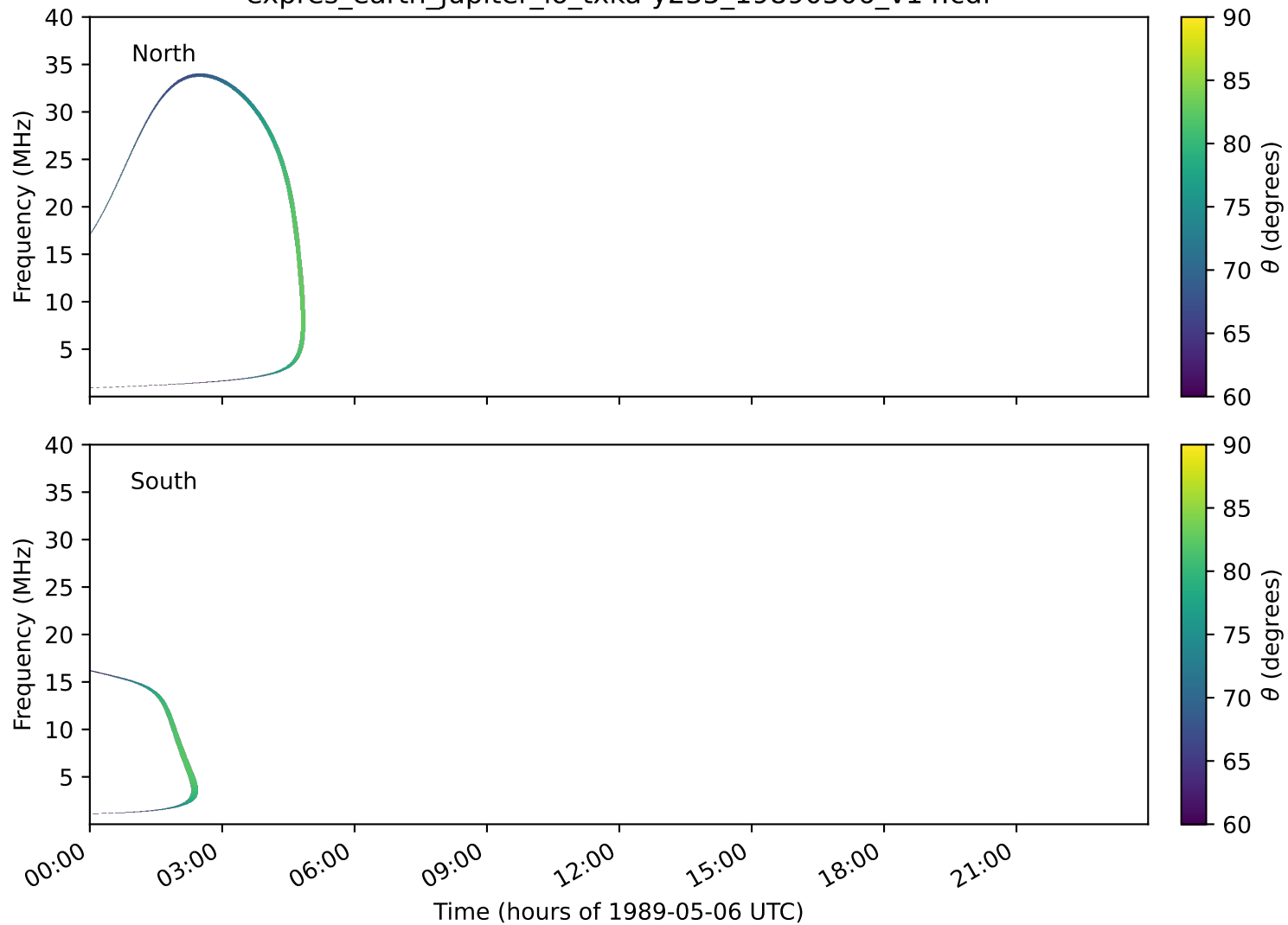
expres_earth_jupiter_io_txka-y235_19890506_v14.cdf
