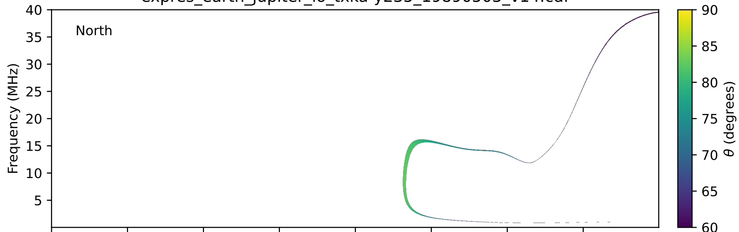
expres_earth_jupiter_io_txka-y235_19890503_v14.cdf
