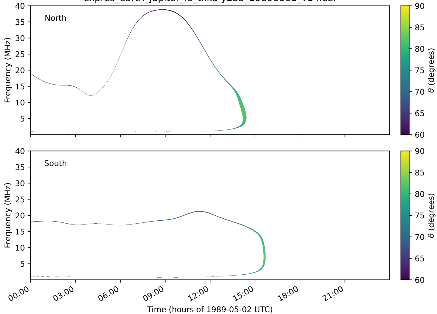
expres_earth_jupiter_io_txka-y235_19890502_v14.cdf
