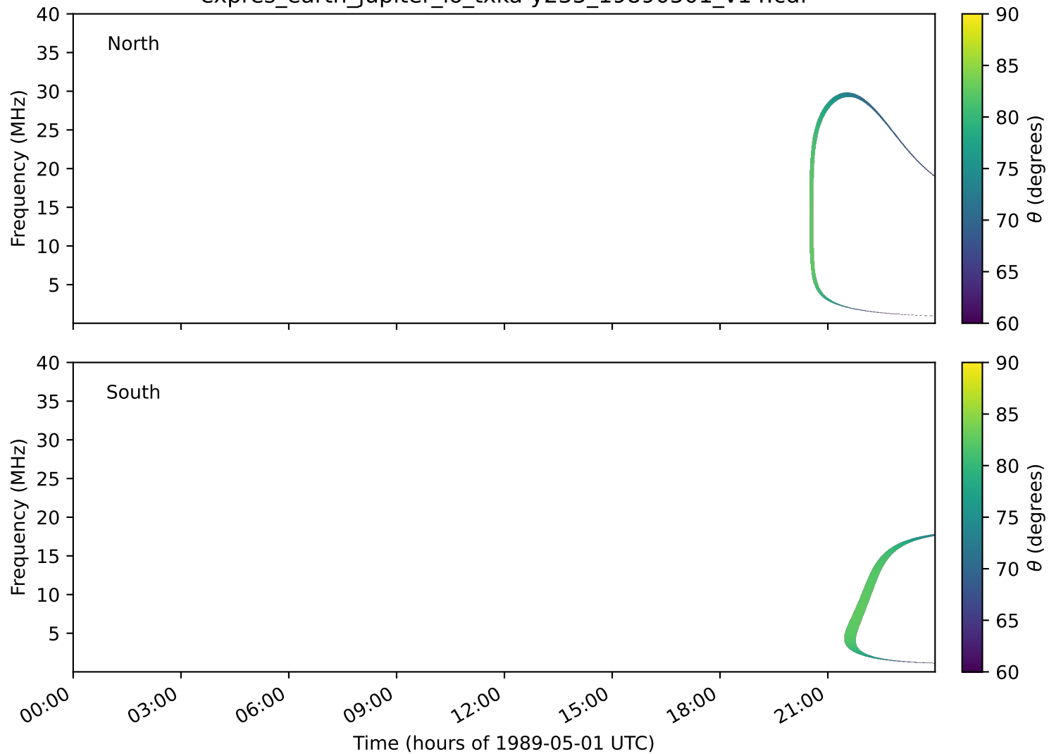
expres_earth_jupiter_io_txka-y235_19890501_v14.cdf
