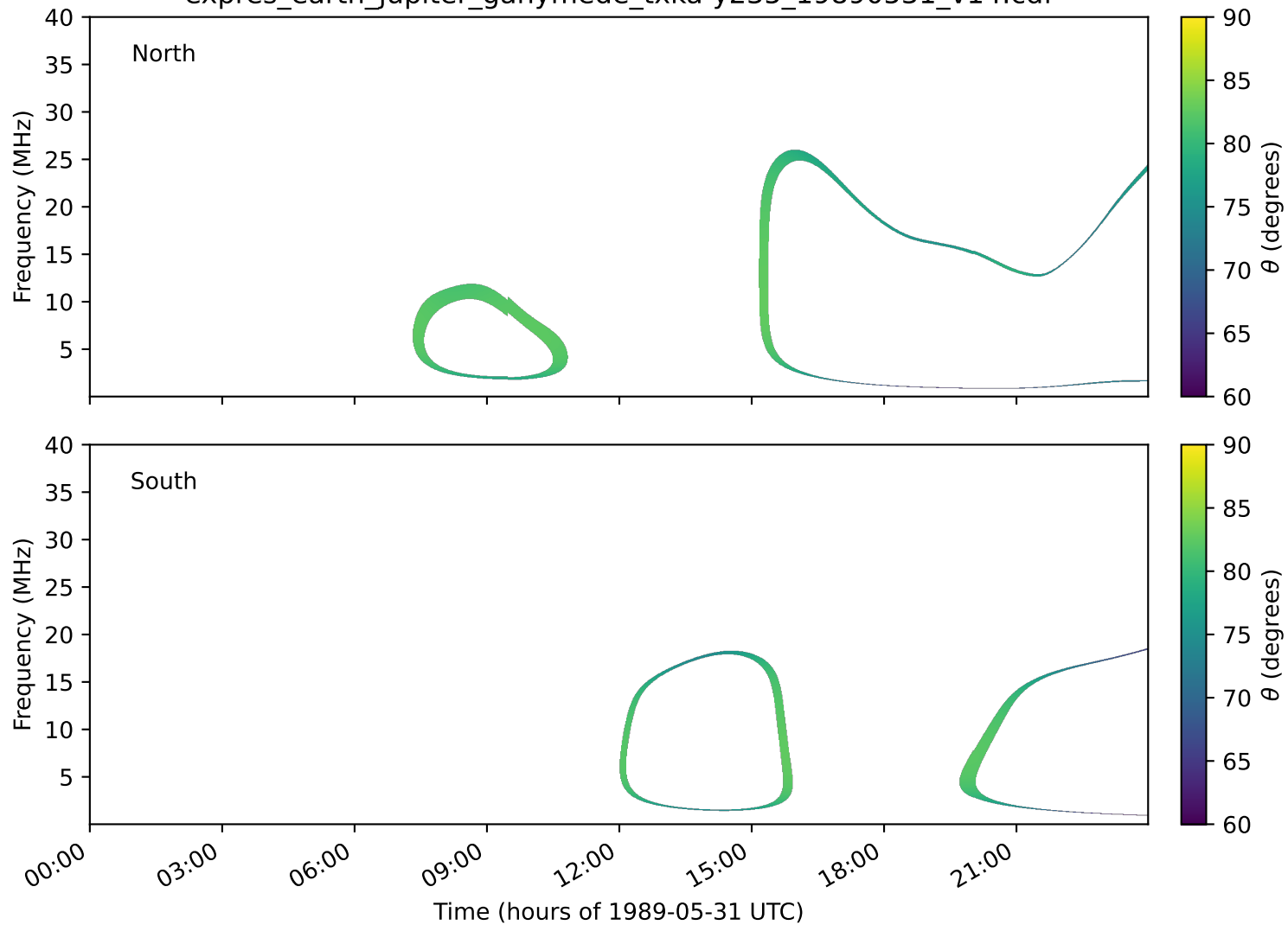
expres_earth_jupiter_ganymede_txka-y235_19890531_v14.cdf
