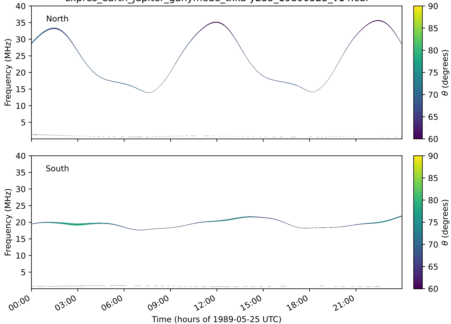
expres_earth_jupiter_ganymede_txka-y235_19890525_v14.cdf
