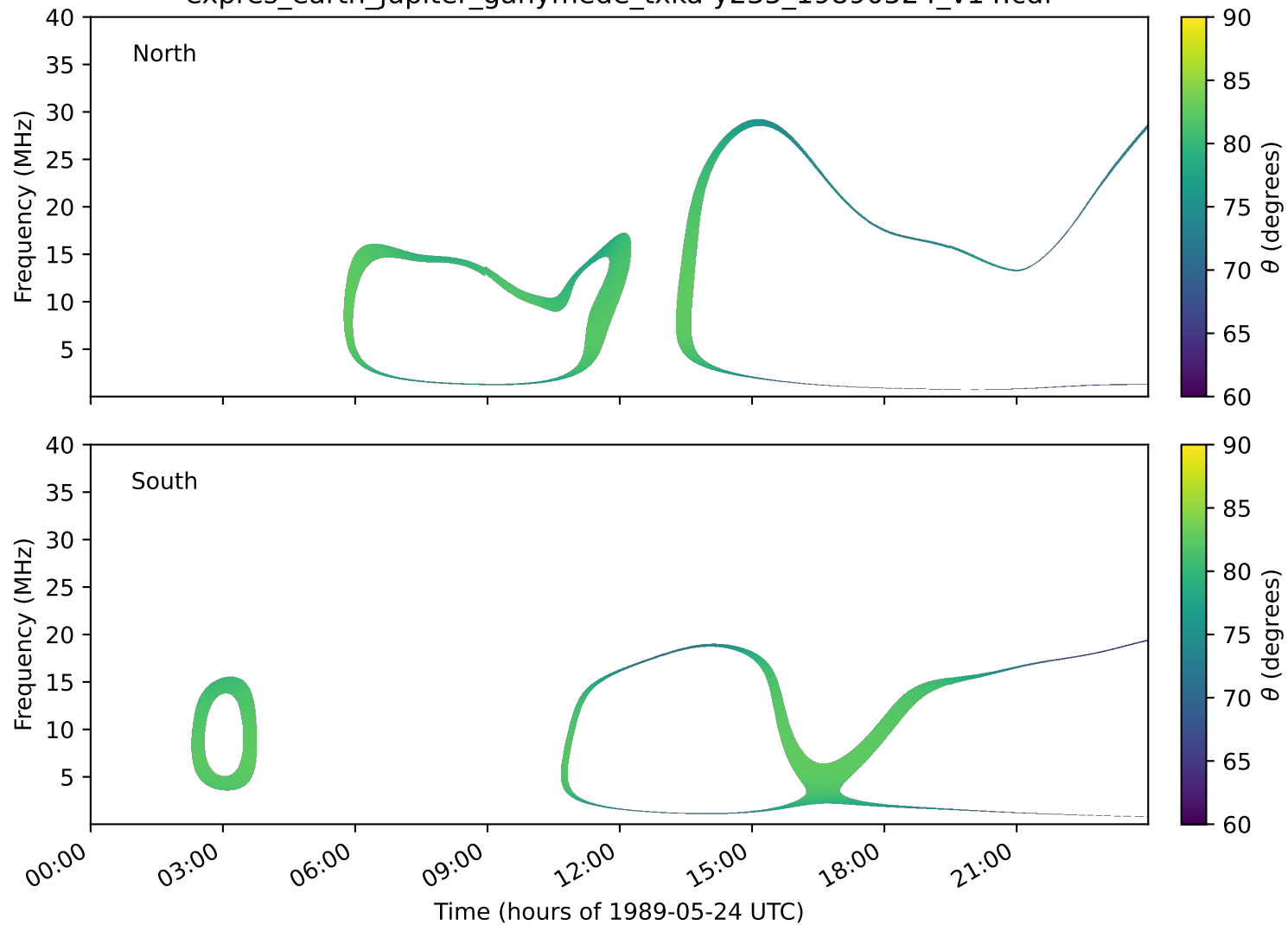
expres_earth_jupiter_ganymede_txka-y235_19890524_v14.cdf
