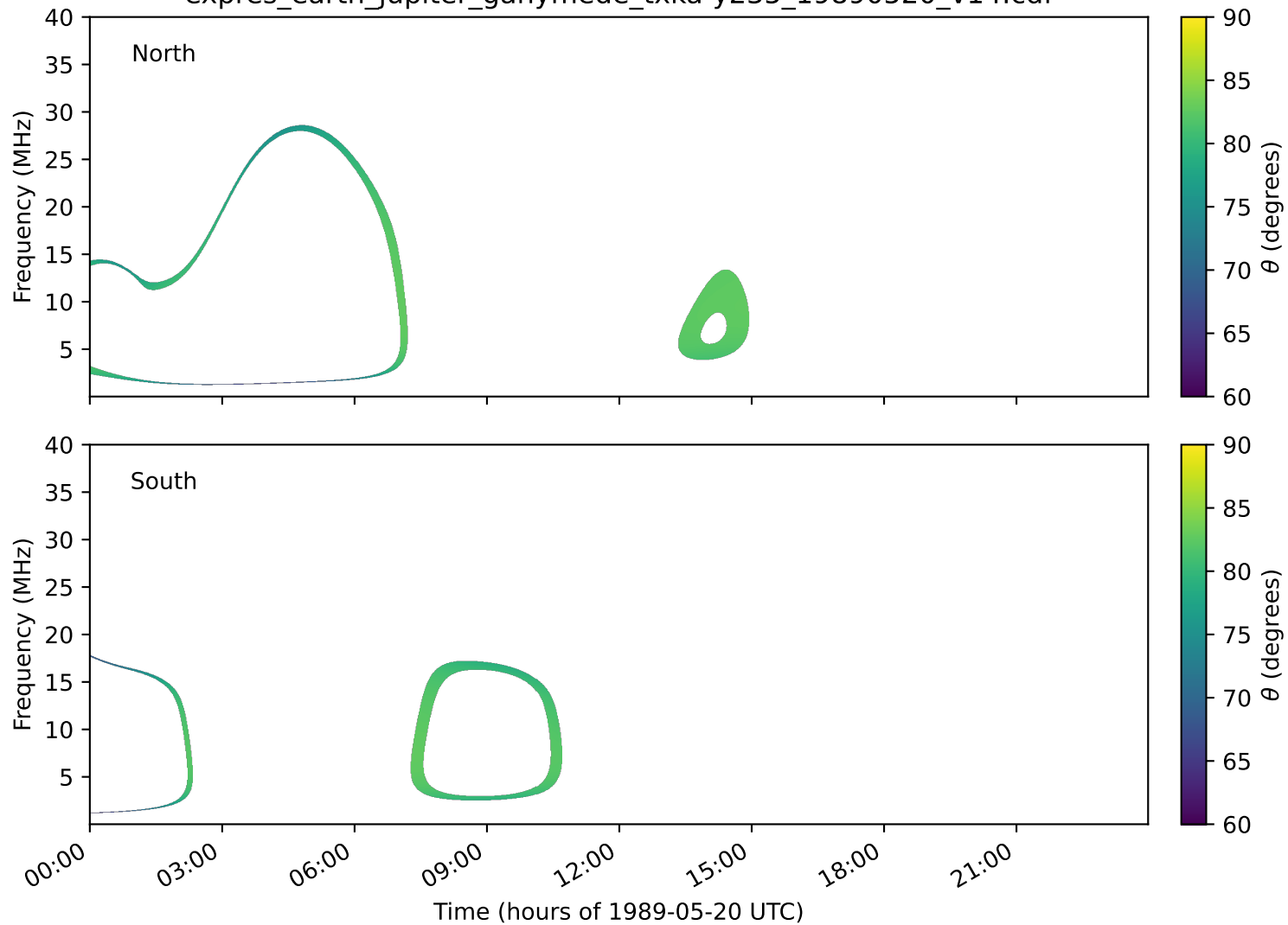
expres_earth_jupiter_ganymede_txka-y235_19890520_v14.cdf
