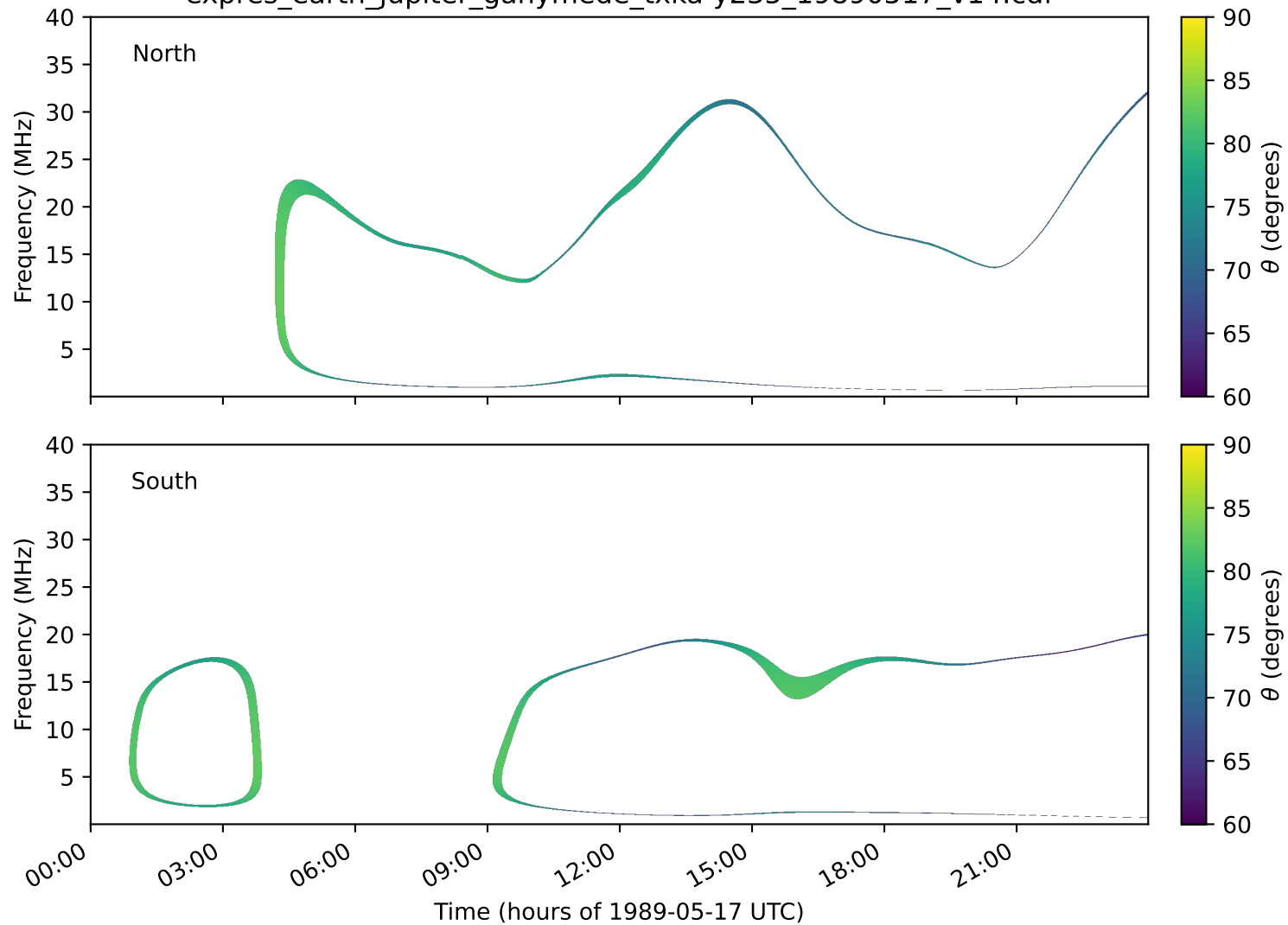
expres_earth_jupiter_ganymede_txka-y235_19890517_v14.cdf
