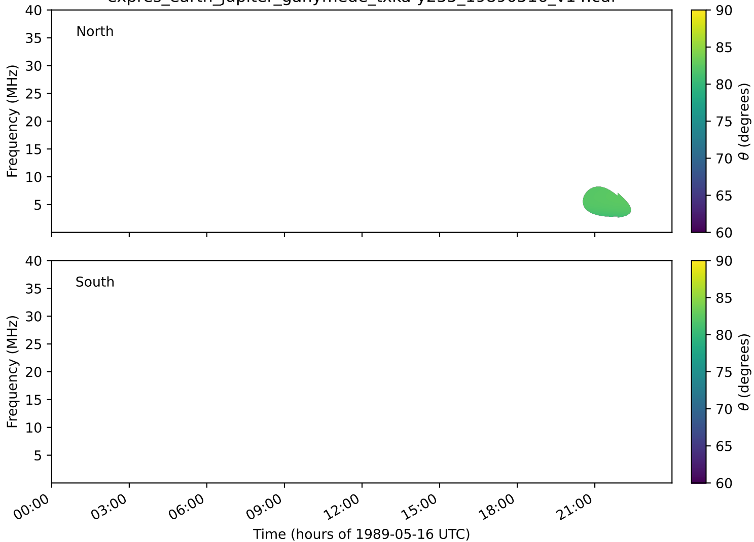
expres_earth_jupiter_ganymede_txka-y235_19890516_v14.cdf
