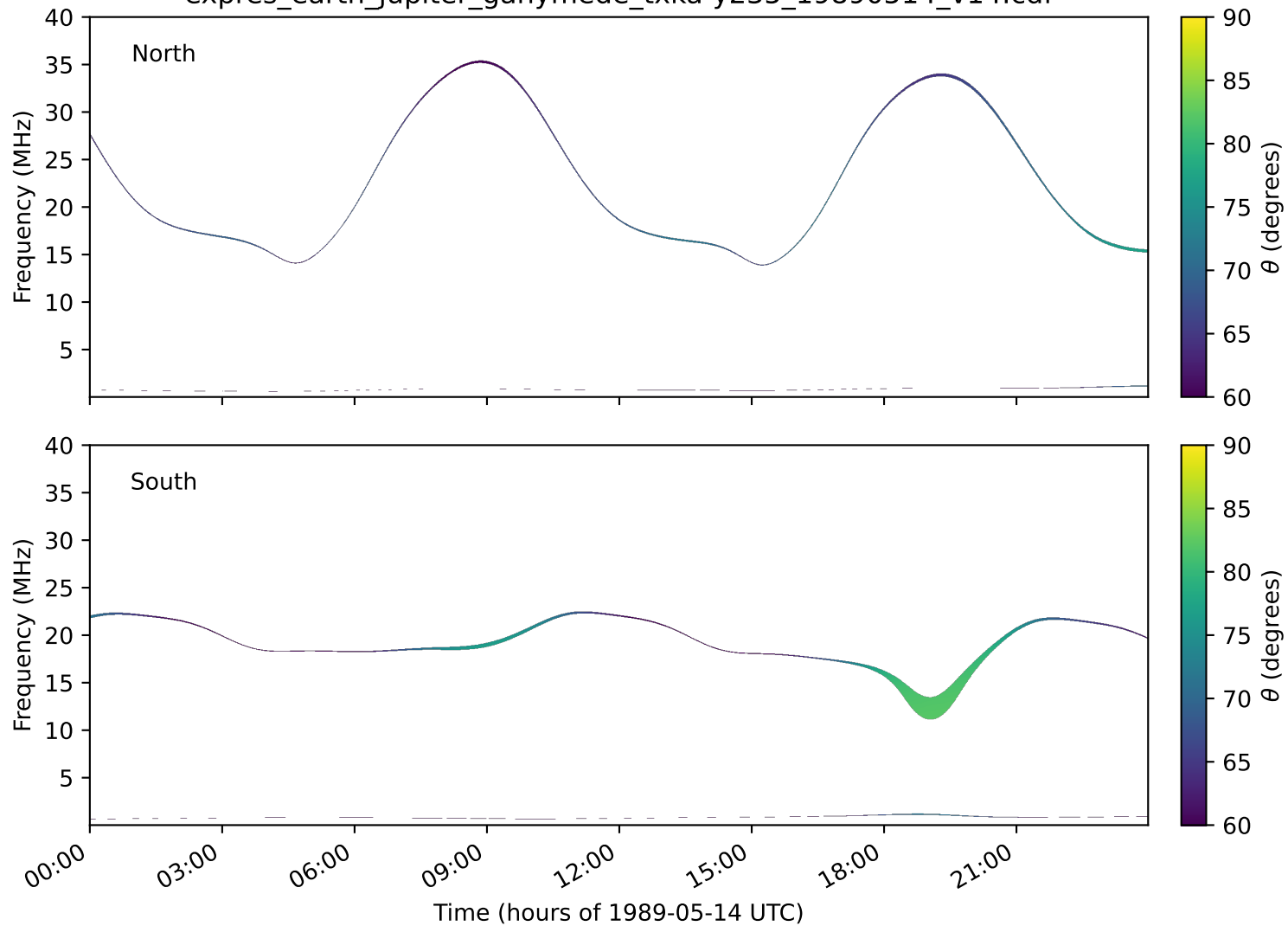
expres_earth_jupiter_ganymede_txka-y235_19890514_v14.cdf
