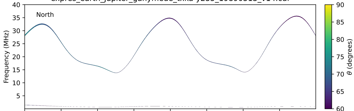
expres_earth_jupiter_ganymede_txka-y235_19890513_v14.cdf
