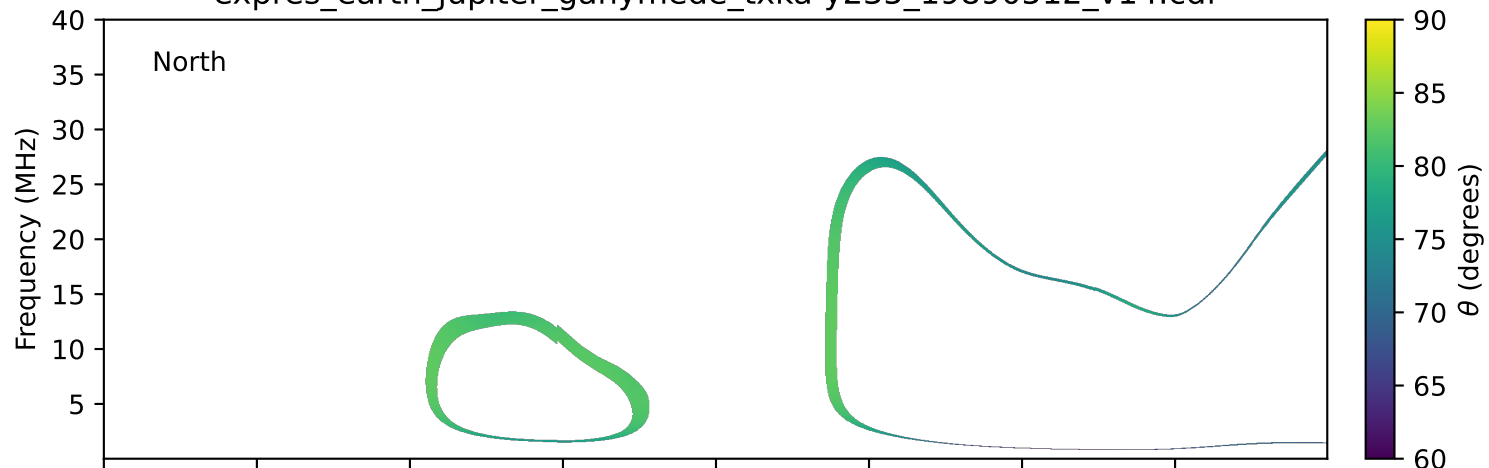
expres_earth_jupiter_ganymede_txka-y235_19890512_v14.cdf
