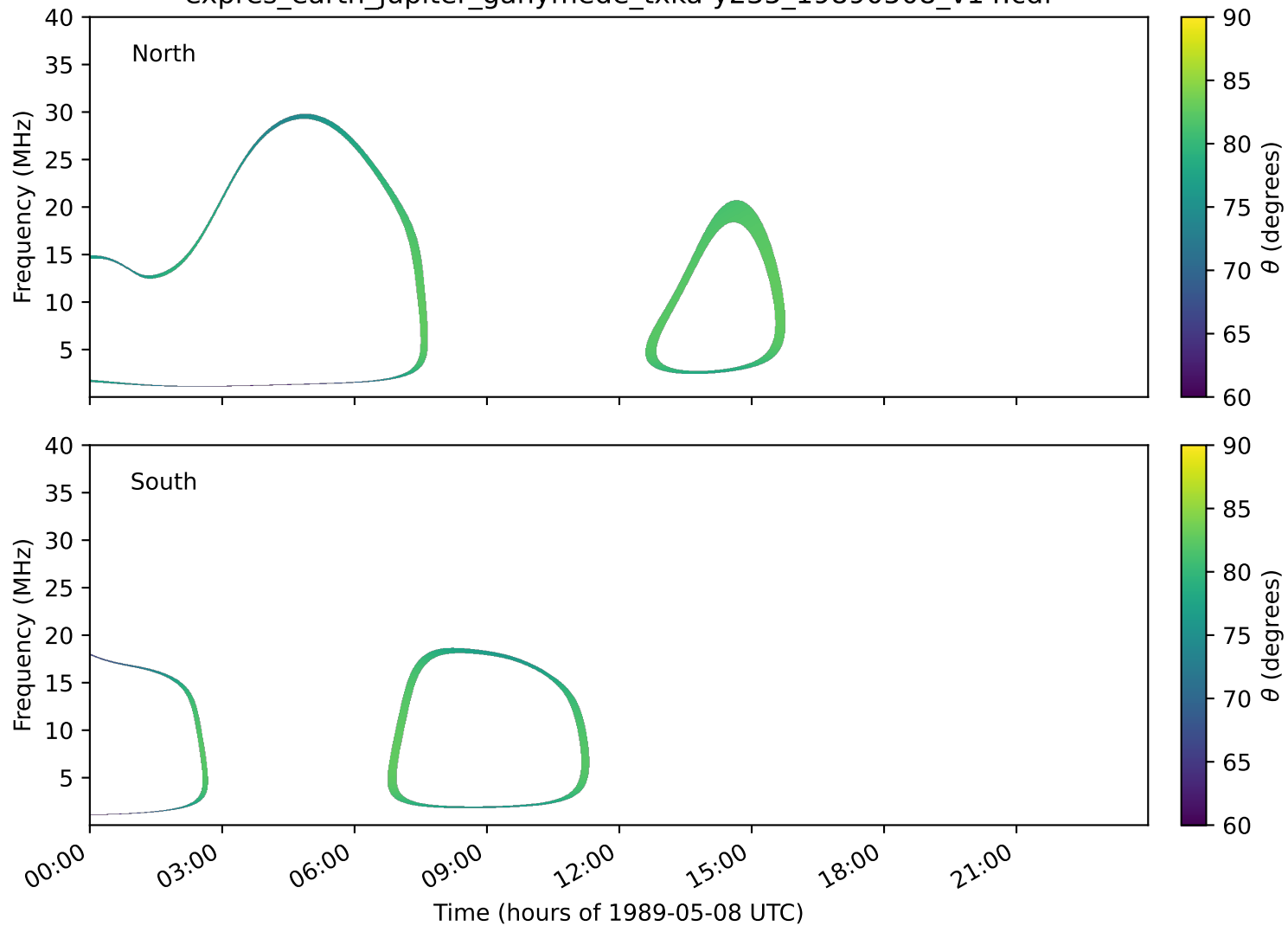
expres_earth_jupiter_ganymede_txka-y235_19890508_v14.cdf
