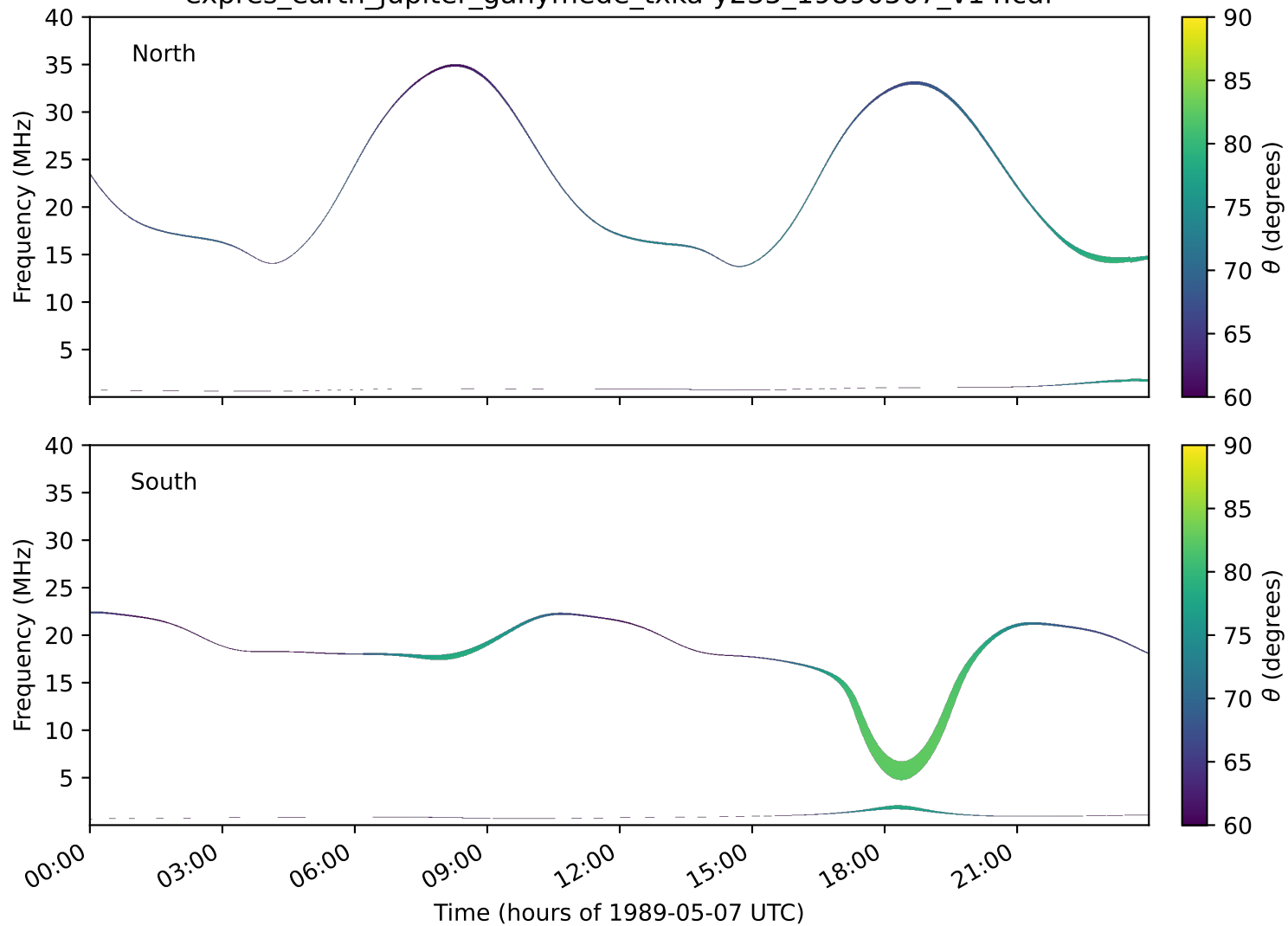
expres_earth_jupiter_ganymede_txka-y235_19890507_v14.cdf
