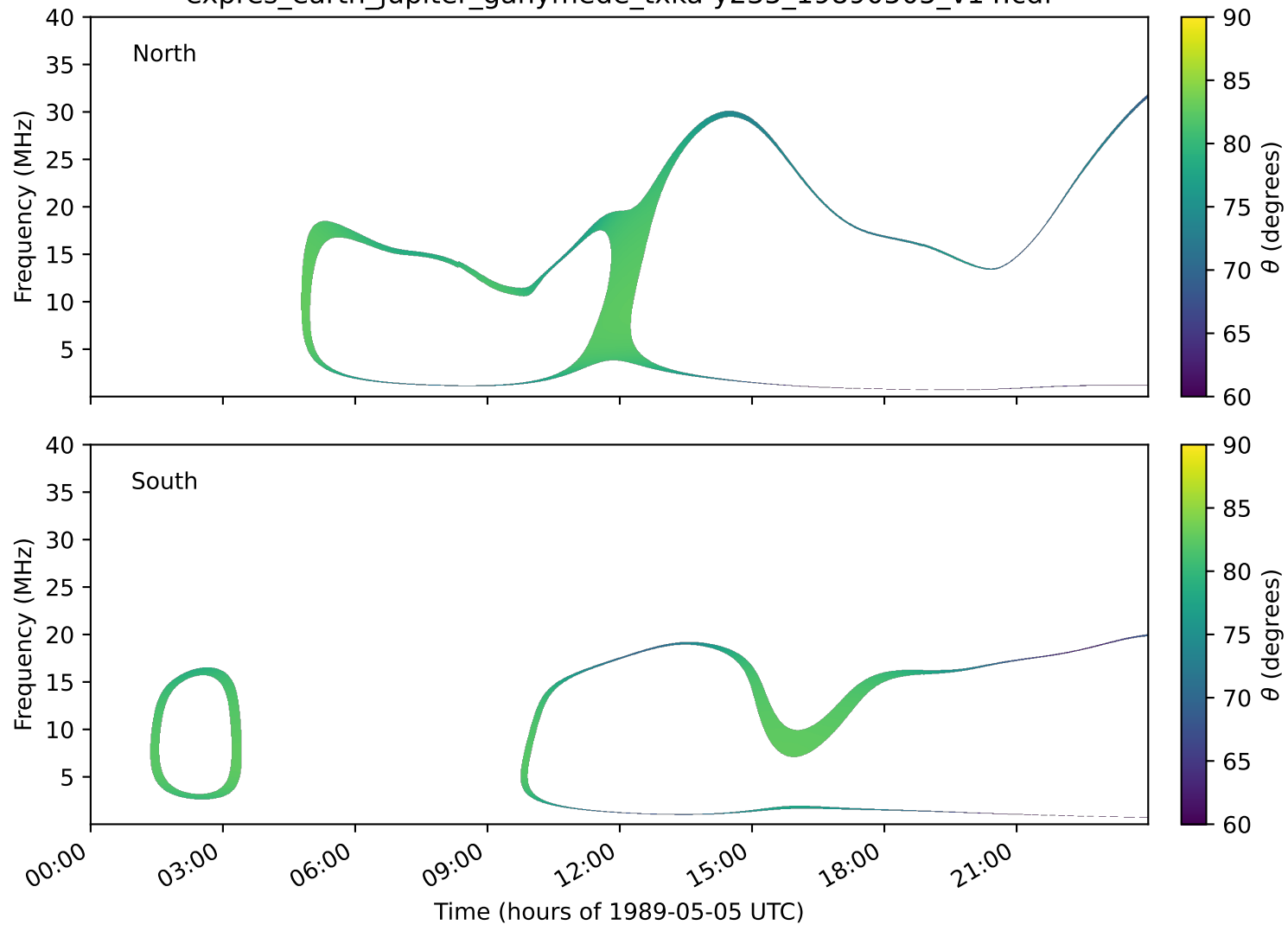
expres_earth_jupiter_ganymede_txka-y235_19890505_v14.cdf
