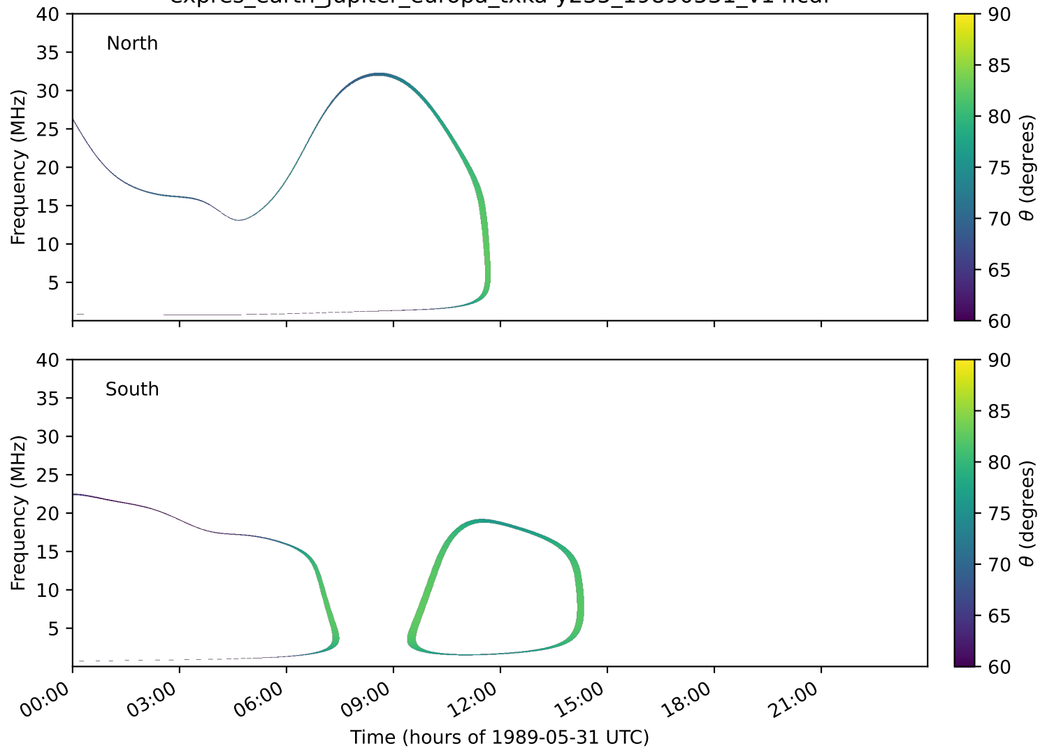
expres_earth_jupiter_europa_txka-y235_19890531_v14.cdf
