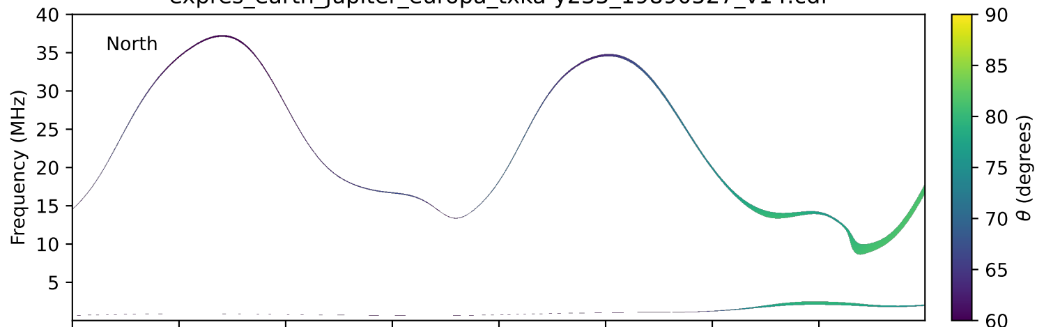
expres_earth_jupiter_europa_txka-y235_19890527_v14.cdf
