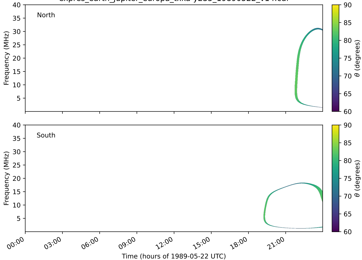
expres_earth_jupiter_europa_txka-y235_19890522_v14.cdf
