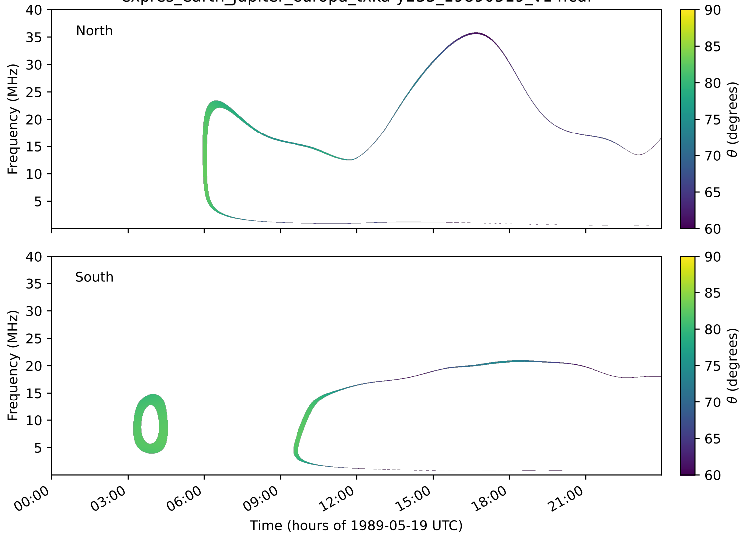
expres_earth_jupiter_europa_txka-y235_19890519_v14.cdf
