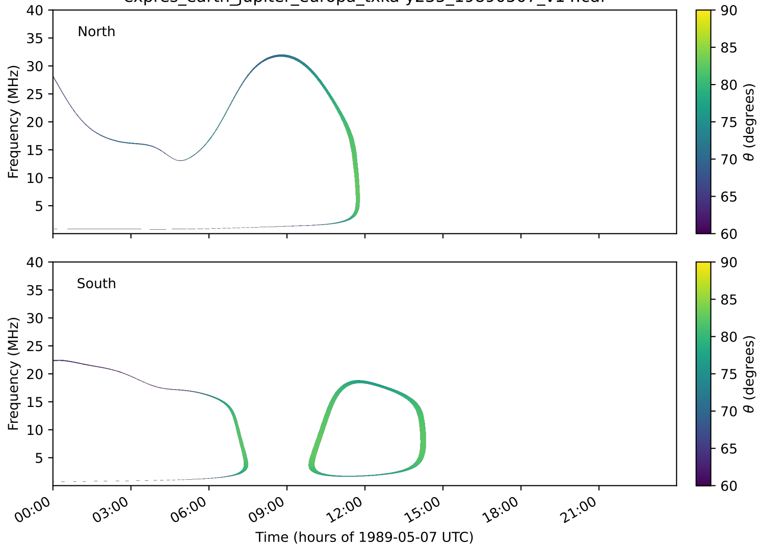
expres_earth_jupiter_europa_txka-y235_19890507_v14.cdf
