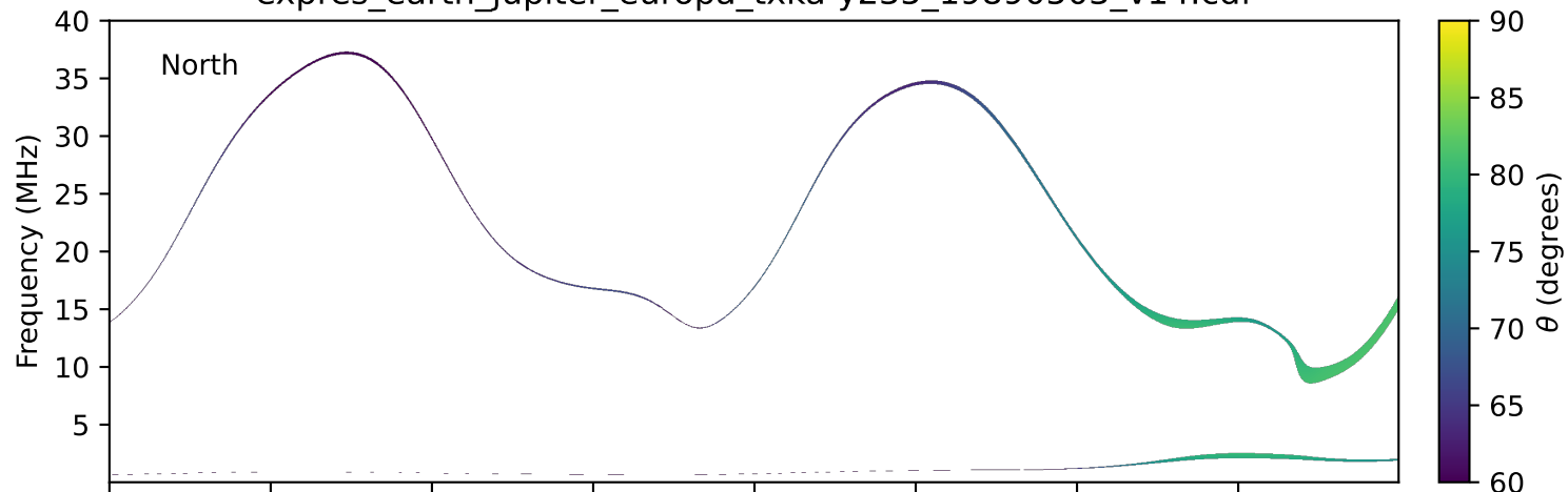
expres_earth_jupiter_europa_txka-y235_19890503_v14.cdf
