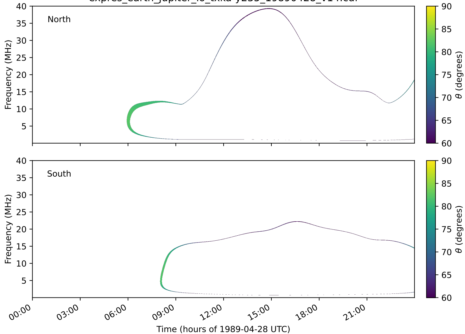
expres_earth_jupiter_io_txka-y235_19890428_v14.cdf
