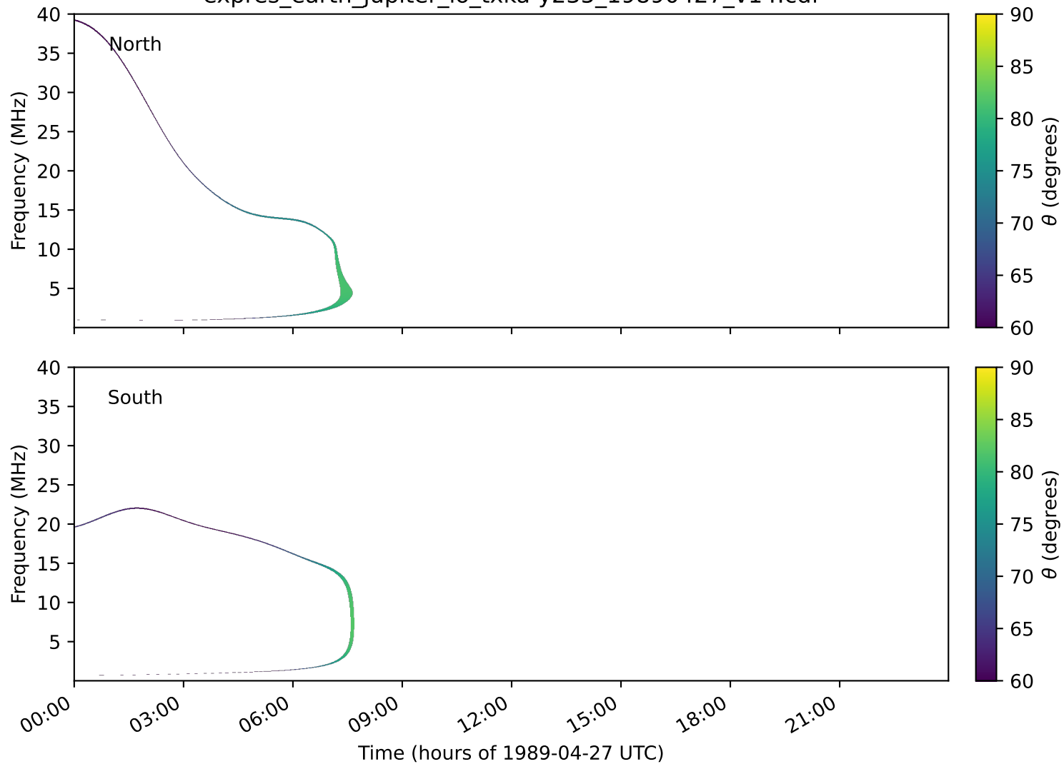
expres_earth_jupiter_io_txka-y235_19890427_v14.cdf
