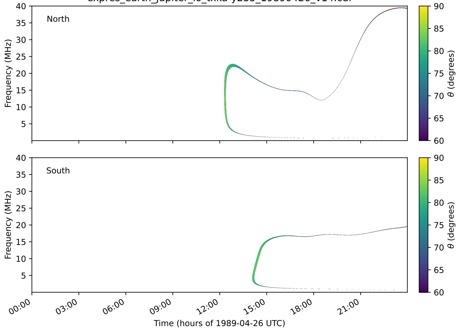
expres_earth_jupiter_io_txka-y235_19890426_v14.cdf
