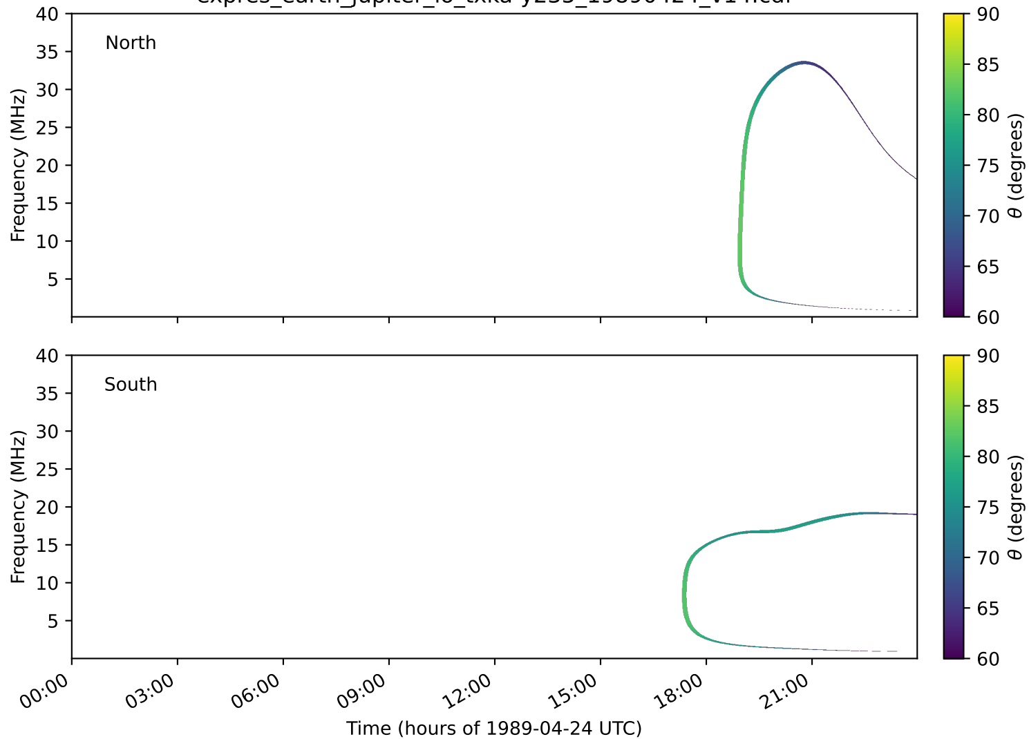
expres_earth_jupiter_io_txka-y235_19890424_v14.cdf
