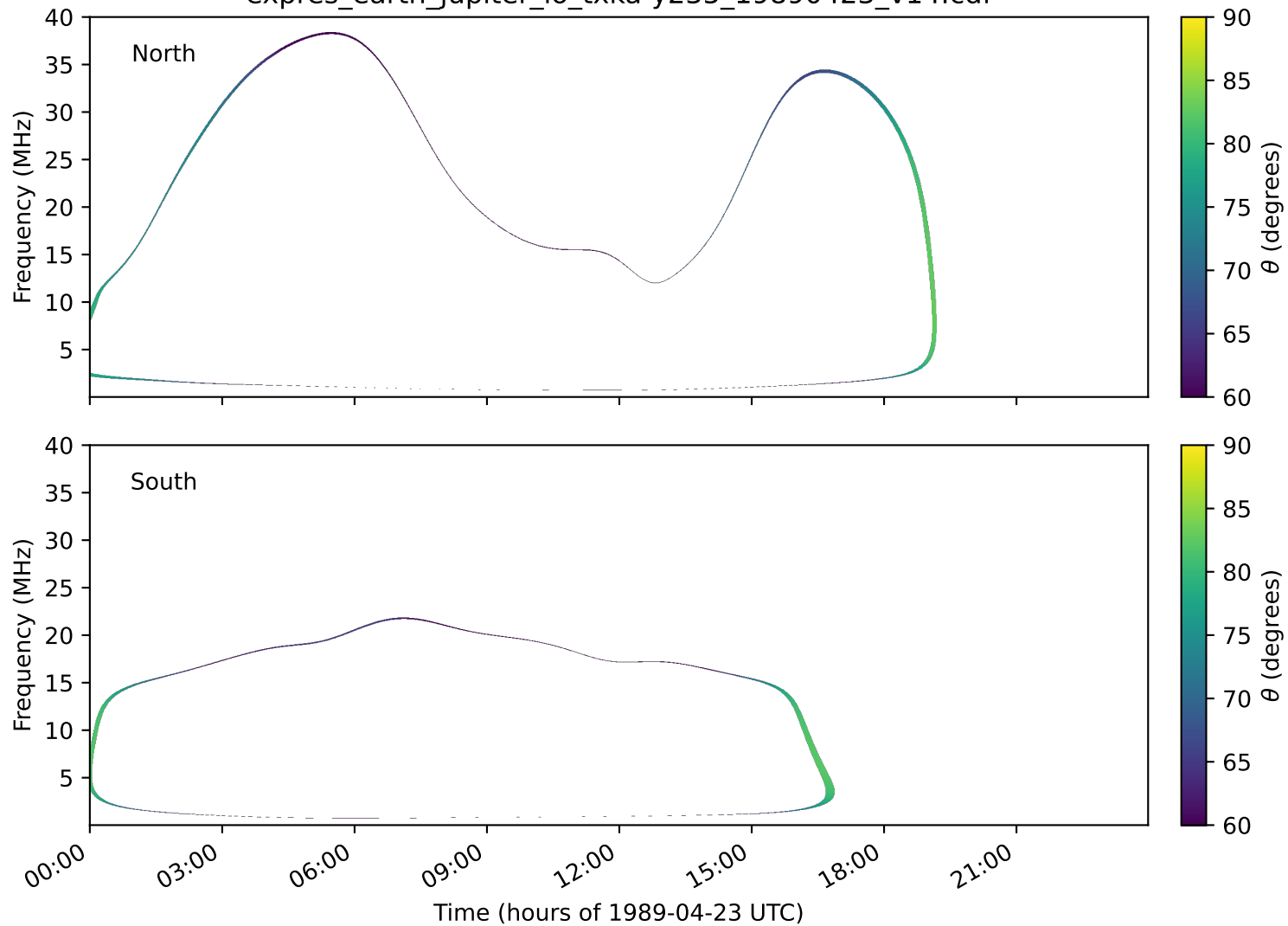
expres_earth_jupiter_io_txka-y235_19890423_v14.cdf
