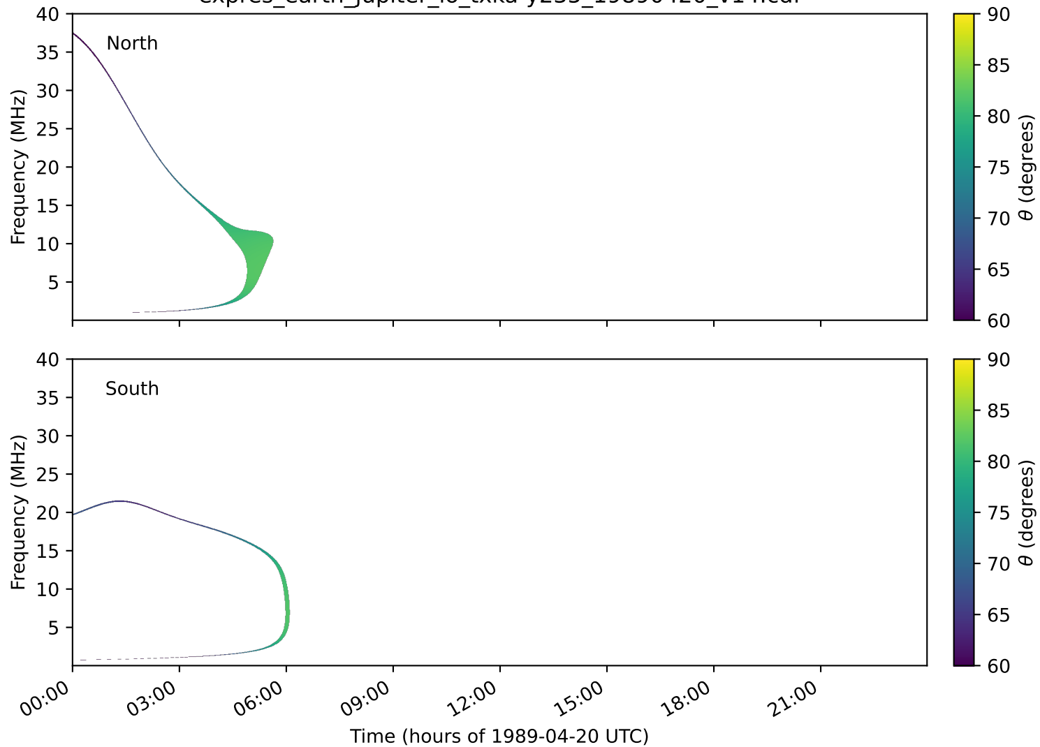
expres_earth_jupiter_io_txka-y235_19890420_v14.cdf
