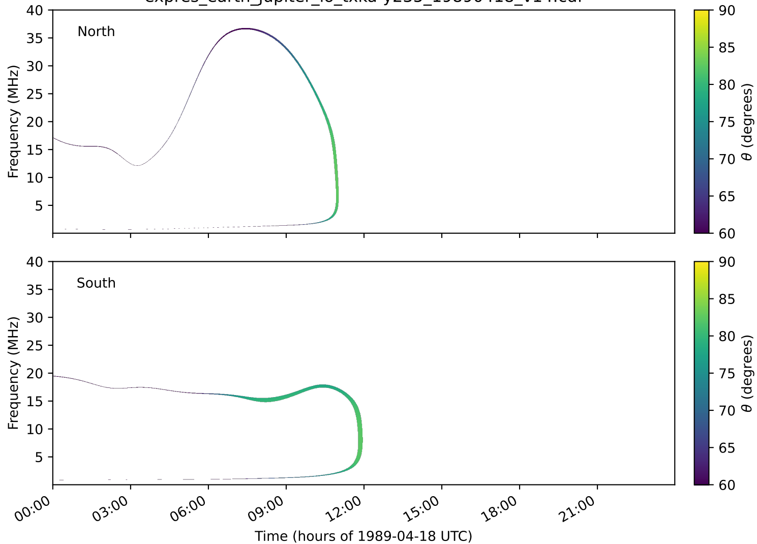
expres_earth_jupiter_io_txka-y235_19890418_v14.cdf
