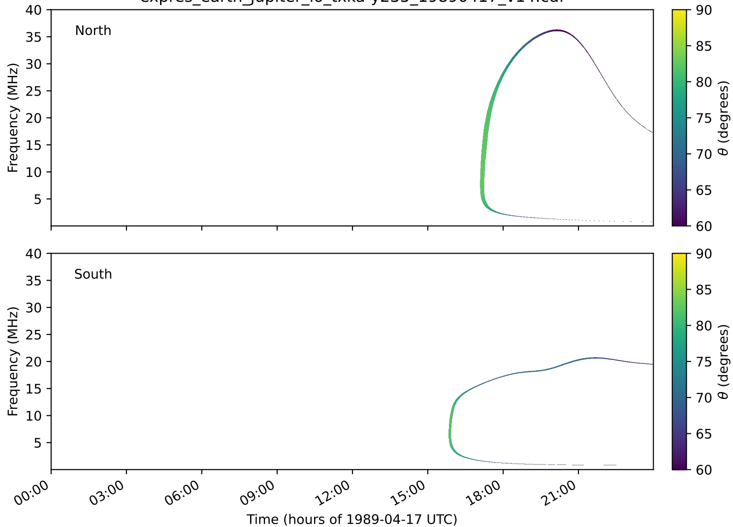
expres_earth_jupiter_io_txka-y235_19890417_v14.cdf
