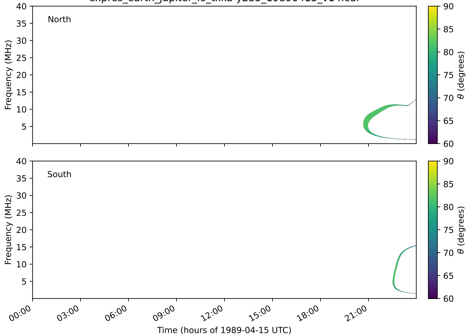
expres_earth_jupiter_io_txka-y235_19890415_v14.cdf
