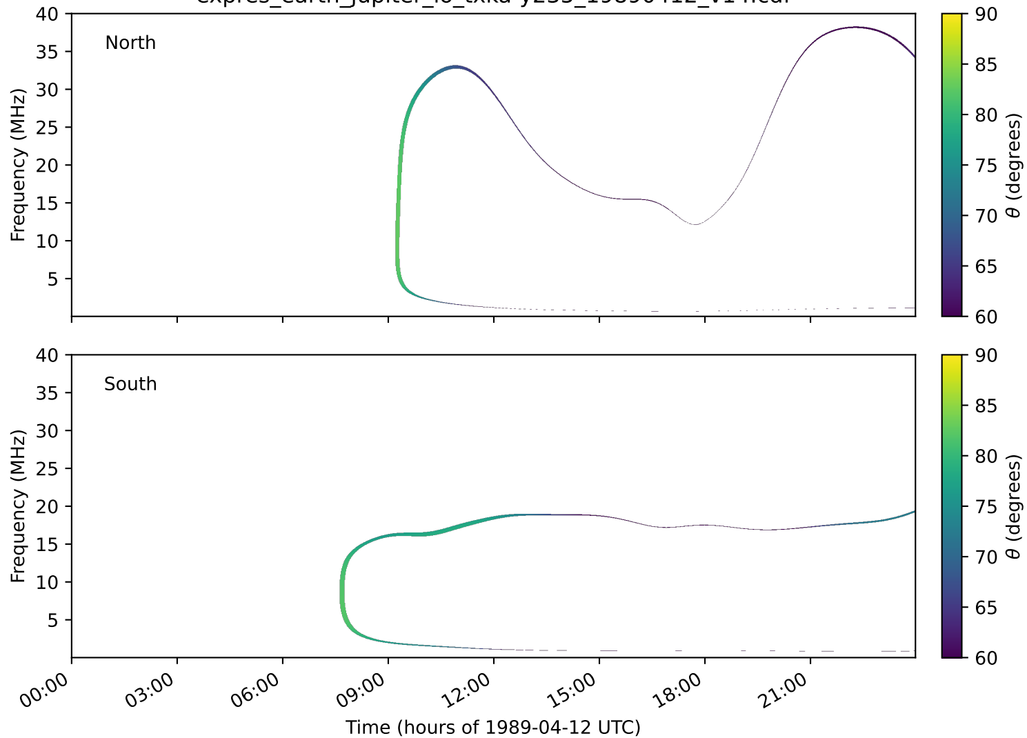
expres_earth_jupiter_io_txka-y235_19890412_v14.cdf
