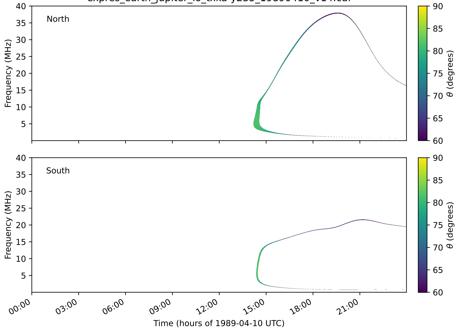
expres_earth_jupiter_io_txka-y235_19890410_v14.cdf
