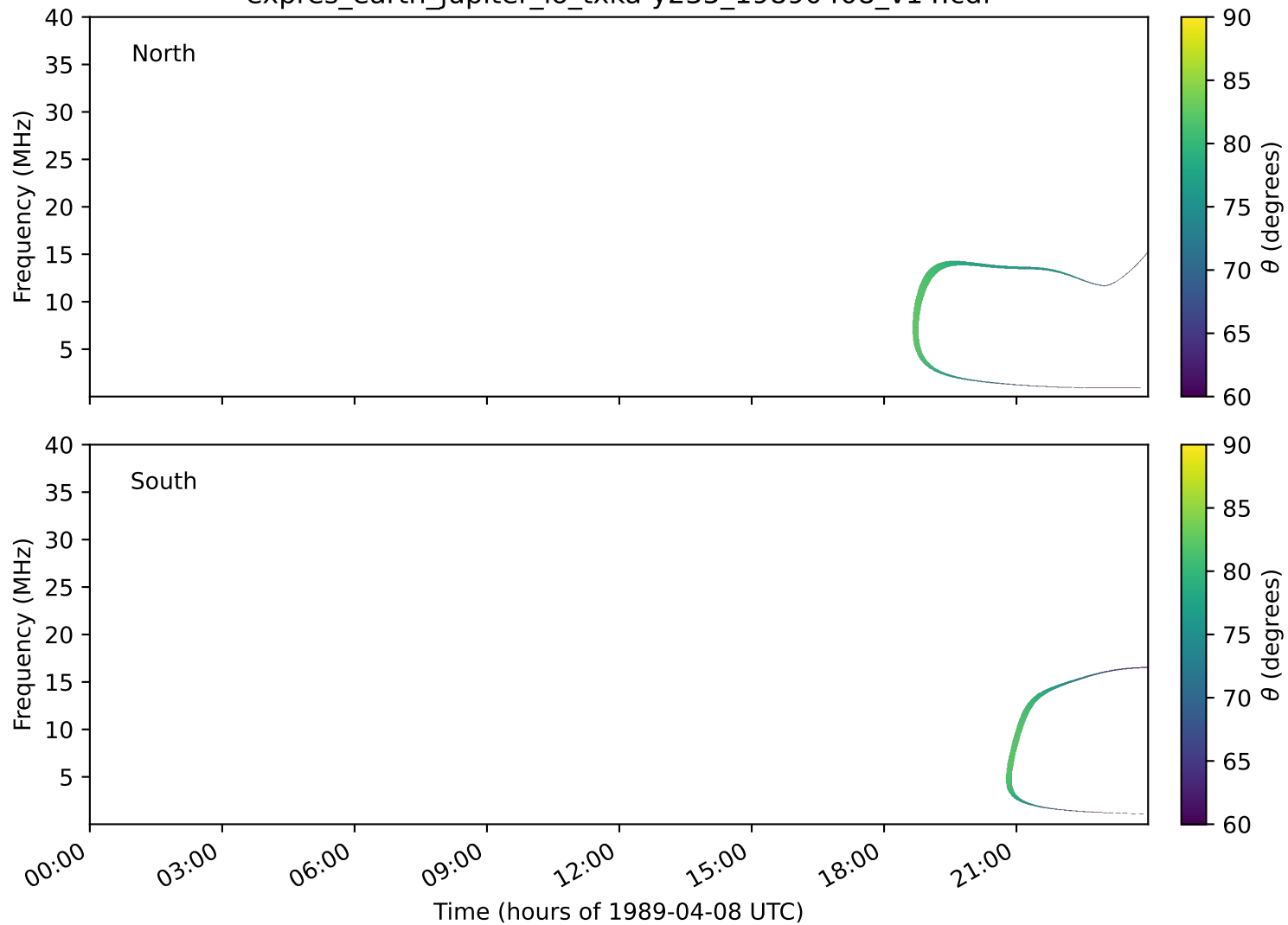
expres_earth_jupiter_io_txka-y235_19890408_v14.cdf
