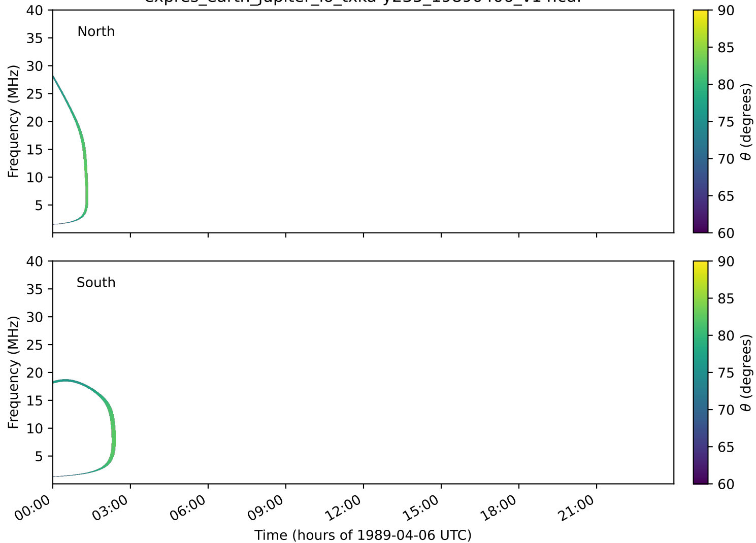
expres_earth_jupiter_io_txka-y235_19890406_v14.cdf
