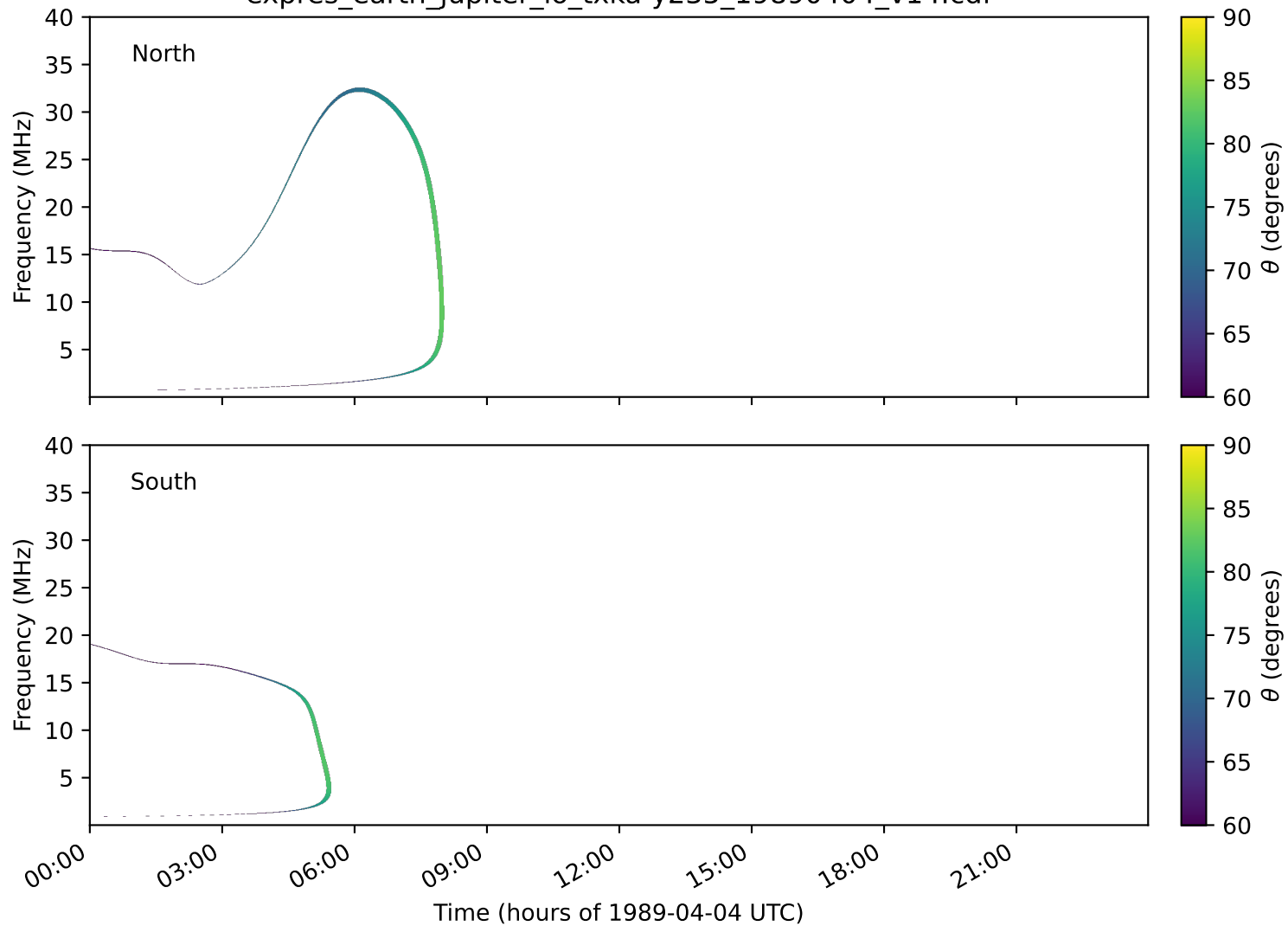
expres_earth_jupiter_io_txka-y235_19890404_v14.cdf
