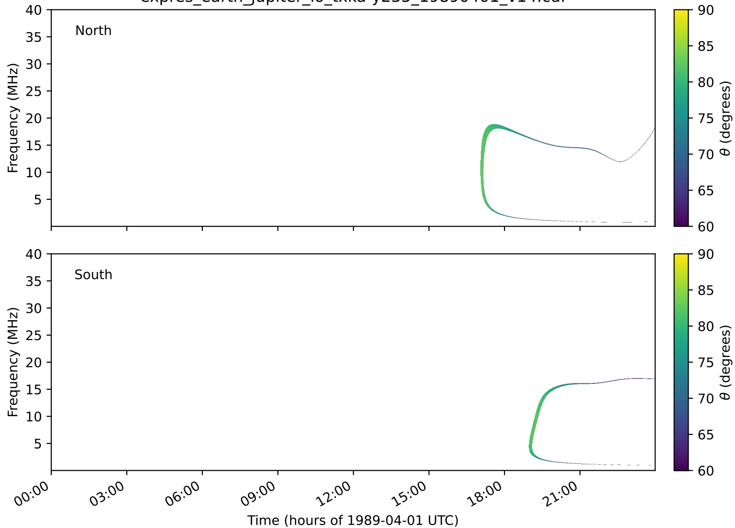
expres_earth_jupiter_io_txka-y235_19890401_v14.cdf
