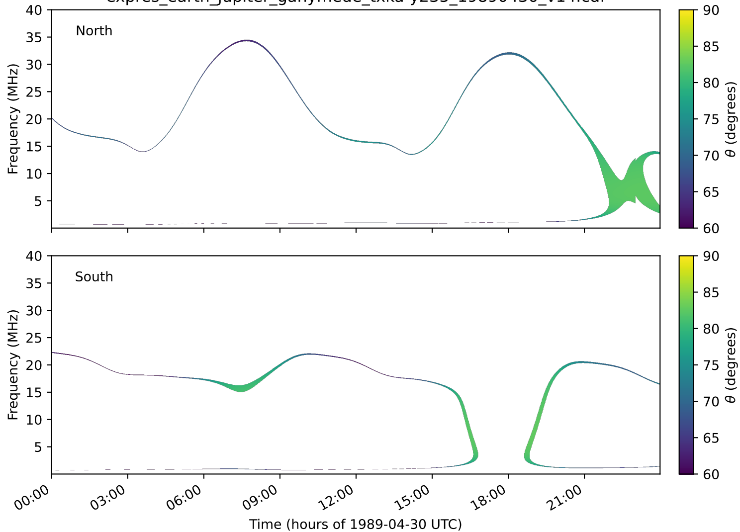
expres_earth_jupiter_ganymede_txka-y235_19890430_v14.cdf
