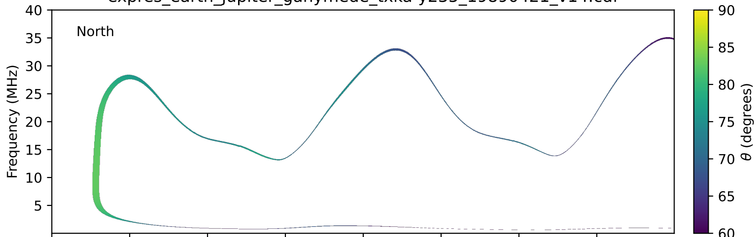
expres_earth_jupiter_ganymede_txka-y235_19890421_v14.cdf
